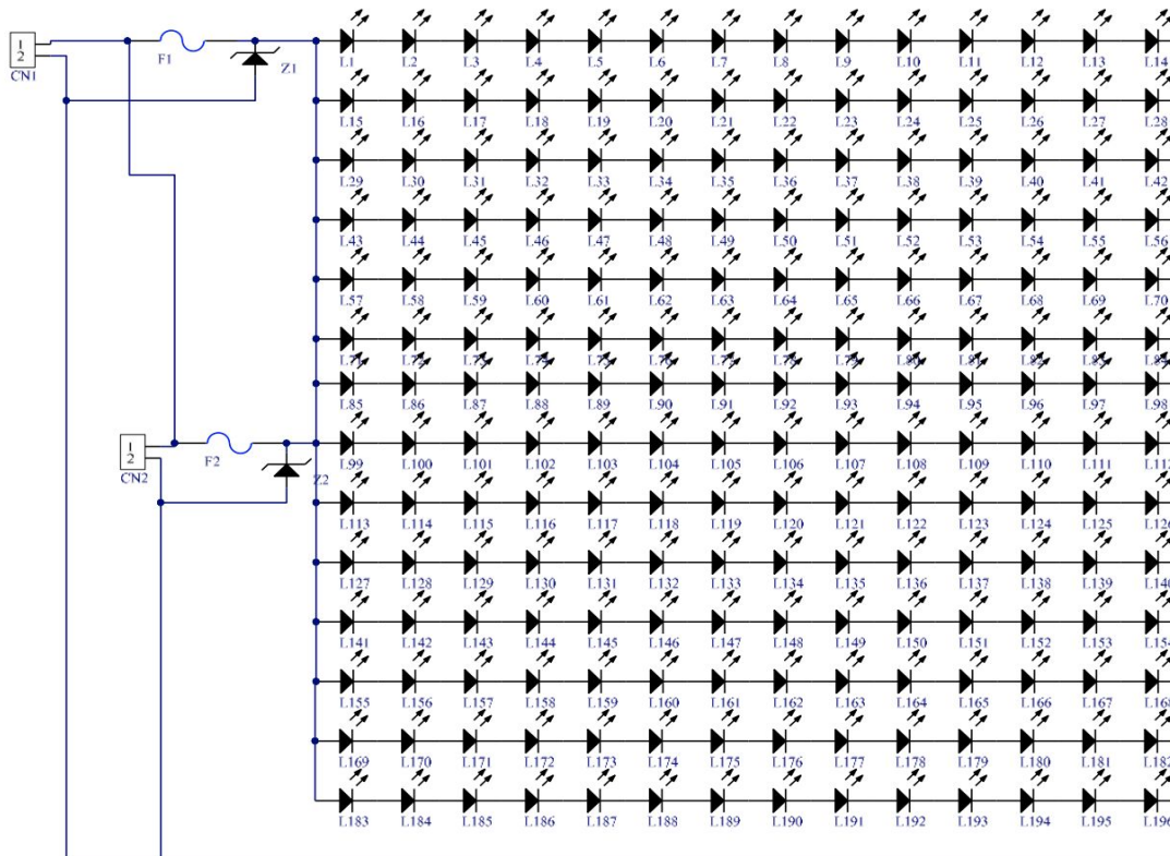
Image 3. Circuit Schematic
